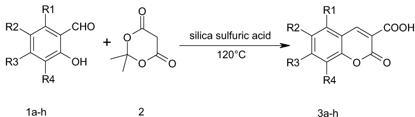
FIGURE 1 One-pot synthesis of coumarin-3-carboxylic acid.
