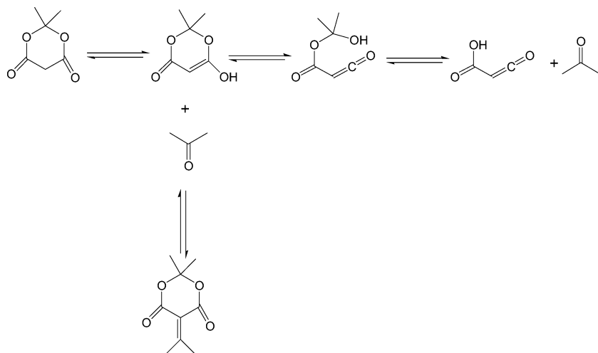
FIGURE 2 Decyclization of Meldrum's acid.
